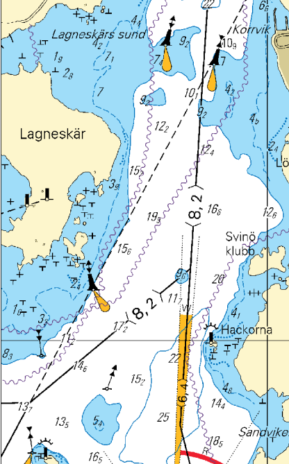
Block for Chart No 2614
